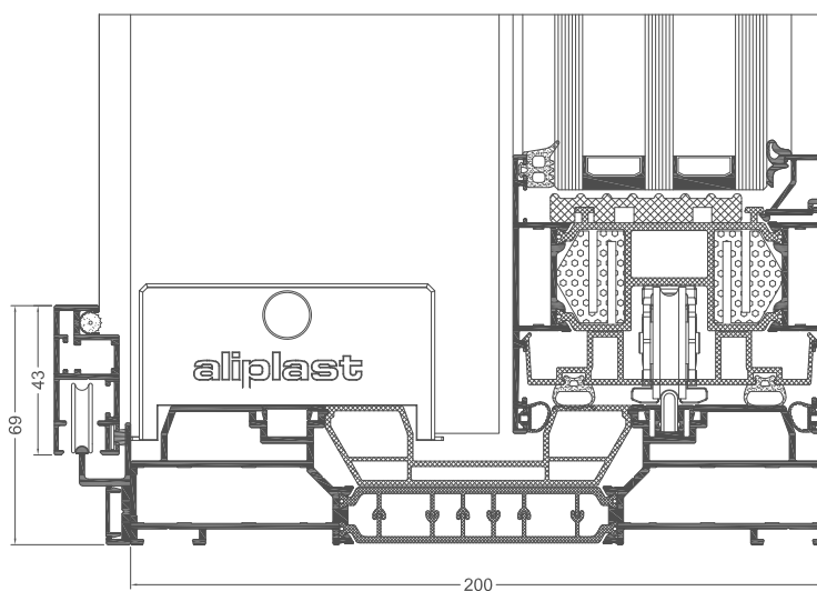
Inferno (MG020 + MG010) + Insect Screen (IS102 + IS104)
