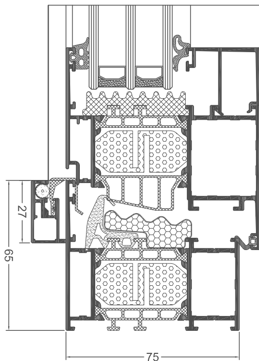
Genesis 75 (GN021 + GN011) + Insect Screen (IS101)
